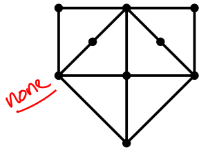
Euler circ.
